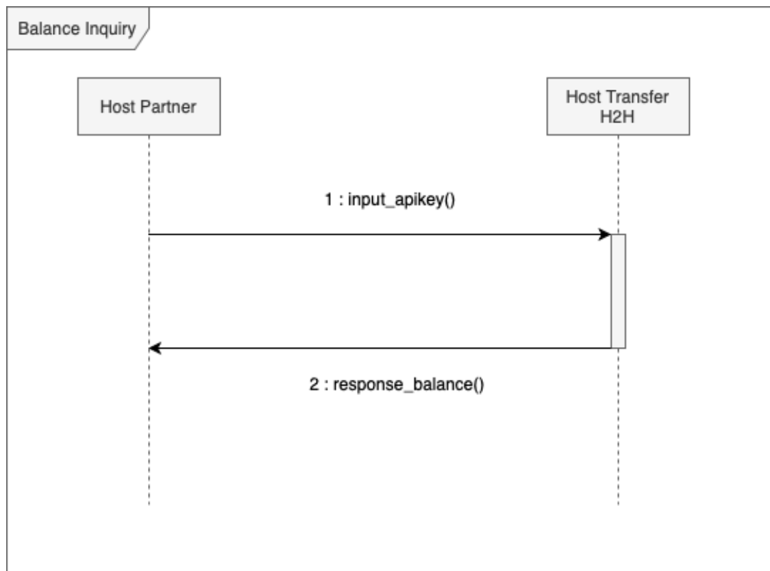
Gambar 2 Sequence Diagram Balance Inquiry
