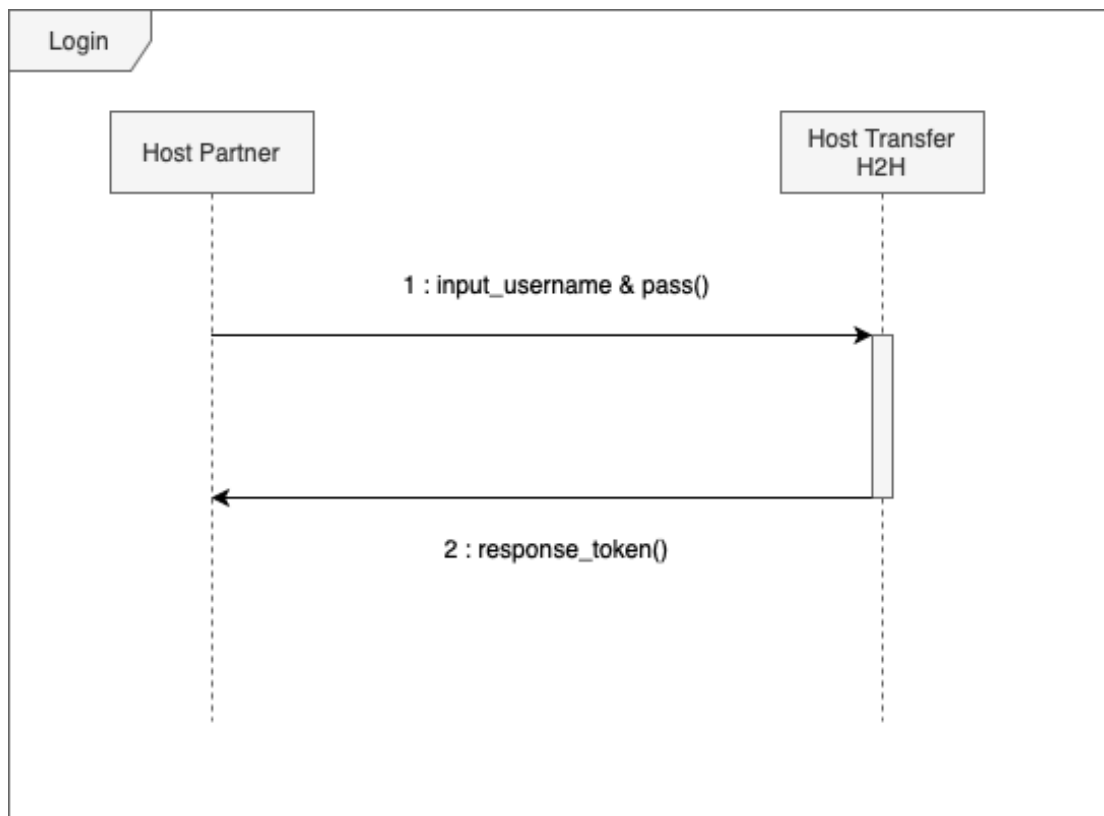
Gambar 1 Sequence Diagram Login
