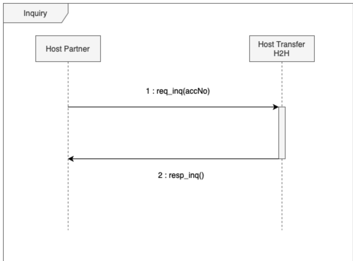
Gambar 4 Sequence Diagram Inquiry
