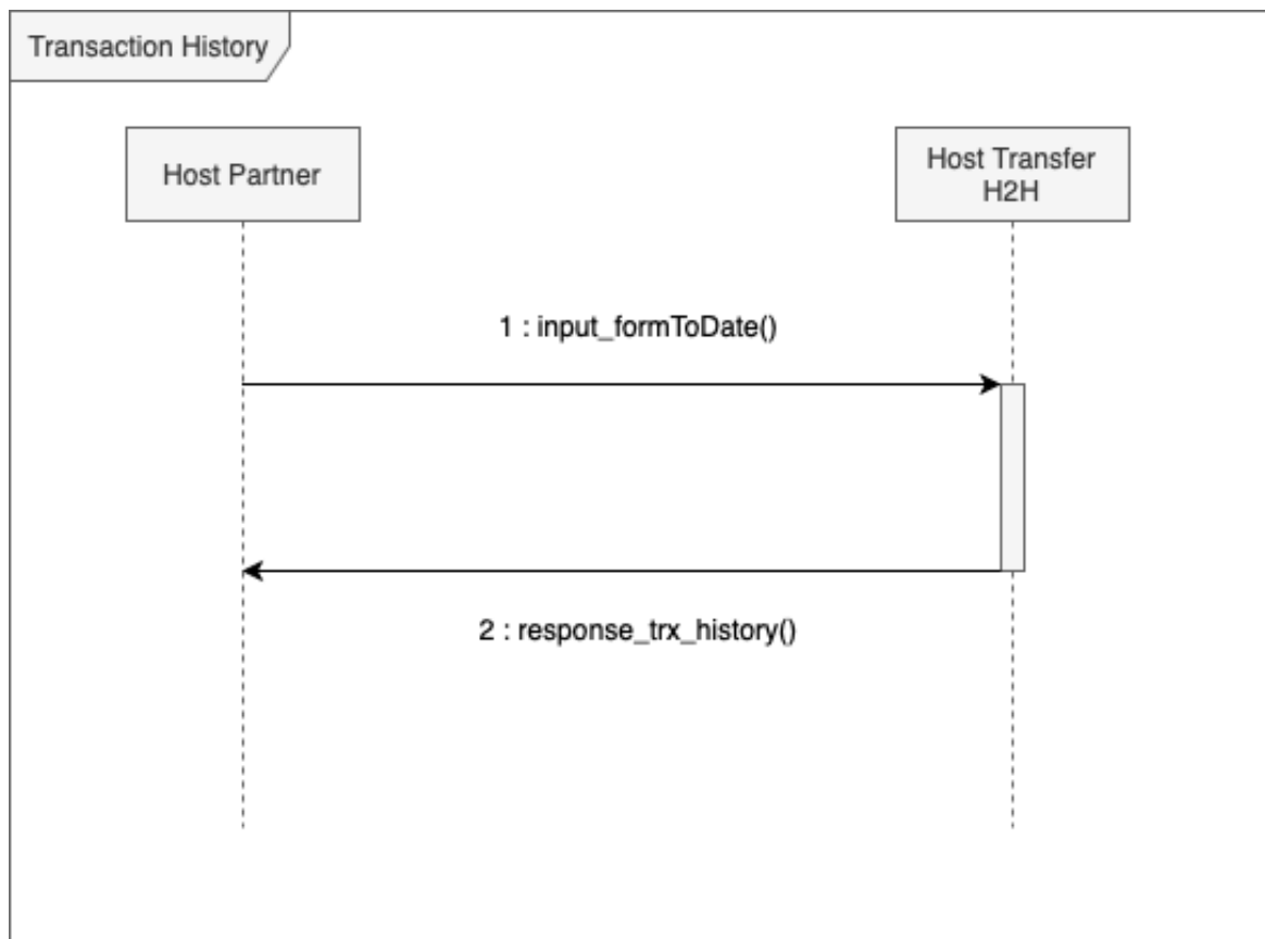
Gambar 3 SequenceDiagram TransactionHistory
