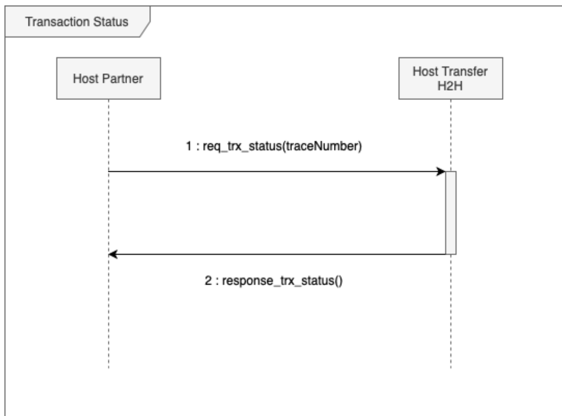
Gambar 6 Sequence Diagram Transaction Status
