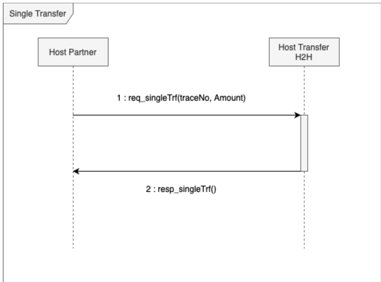
Gambar 5 Sequence Diagram Single Transfer
